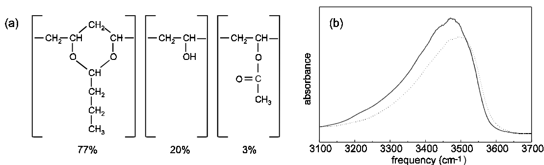
FIGURE 9.2. (a) Chemical structure of poly(vinylbutyral). (b) Infrared absorption spectra of poly(vinylbutyral) from 3100 to 3700 \text{cm}^{-1} at room temperature (dotted line) and at 15 K (solid line).
