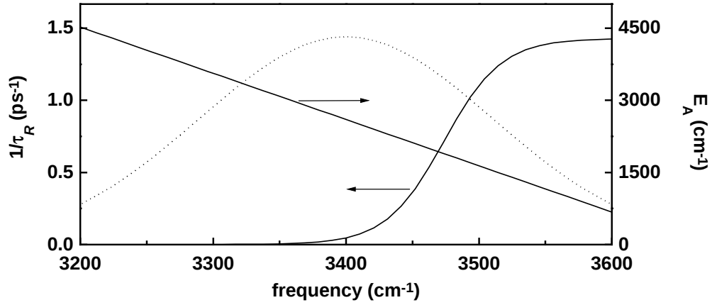
FIGURE 5.4. Frequency dependence of the activation energy E_A(v_{OH}) and the decay constant \tau_R(v_{OH}) . The dotted curve shows the Gaussian v_{OH} absorption band used in the calculation.
