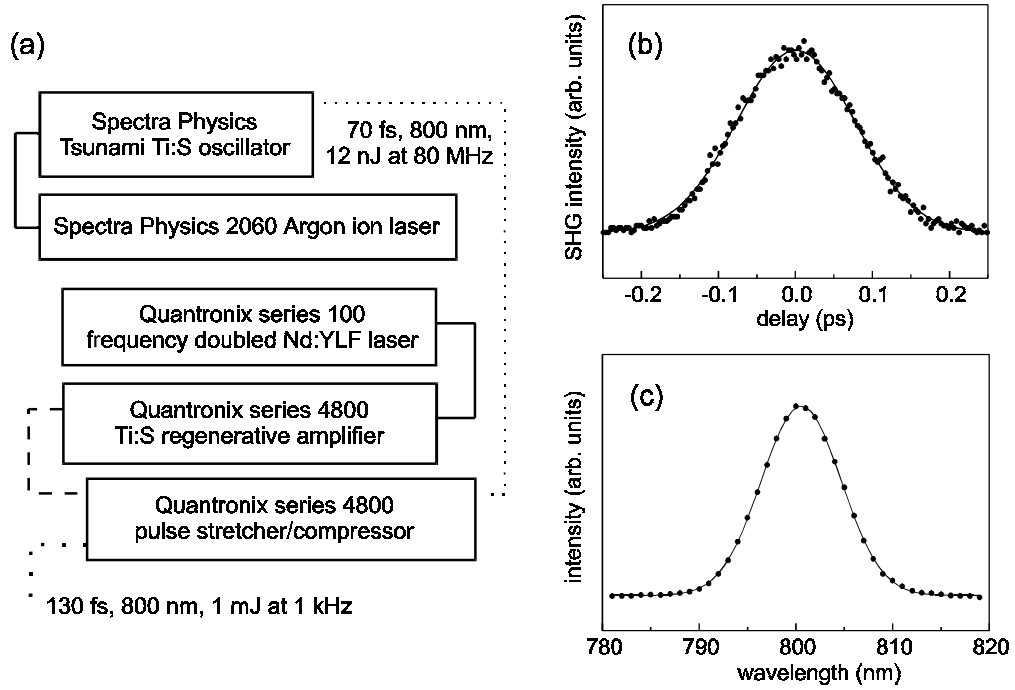
FIGURE 2.1. (a) The amplified Ti:sapphire laser system. (b) Autocorrelation trace of the compressed amplifier output, recorded in a 100 \mu\text{m} thick BBO crystal. The solid curve is a Gaussian with a FWHM of 181 fs. (c) Power spectrum of the pulses, recorded with a scanning monochromator. The solid curve is a Gaussian with a FWHM of 9.7 nm.
