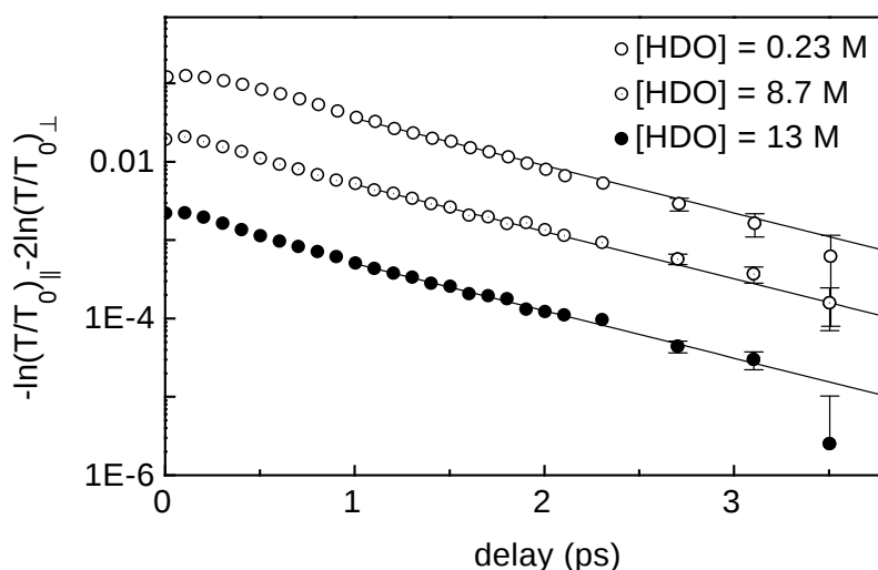
FIGURE 8.3. Rotation-free excited-state absorption -\ln(T/T_0)_{||} - 2\ln(T/T_0)_{\perp} recorded in HDO:D 2 O solutions with three different HDO concentrations. The pump frequency and probe frequencies are \nu_{pu} = 3400 \text{ cm}^{-1} and \nu_{pr} = 3150 \text{ cm}^{-1} , respectively. The transients for [\text{HDO}] = 8.7 \text{ M} and [\text{HDO}] = 13 \text{ M} have been vertically displaced for clarity. The solid lines represent a single-exponential decays with a time constant of 720 fs.
