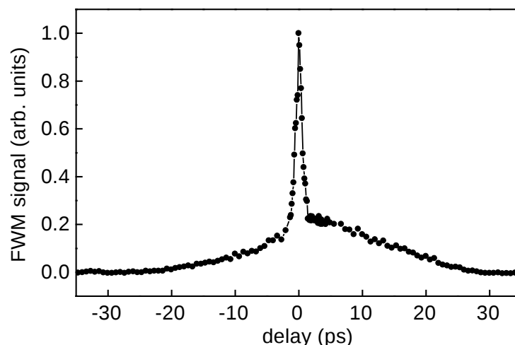
FIGURE 9.4. Integrated four-wave mixing intensity as a function of delay between \mathbf{k}_1 and \mathbf{k}_2 , at an excitation wavelength of 3.0\ \mu\text{m} in a 100\ \mu\text{m} thick sample consisting of a 2.2\ \text{mol/l} solution of methanol in bromoform at room temperature. The signal consists of a symmetric coherence spike superposed on a broad background.
